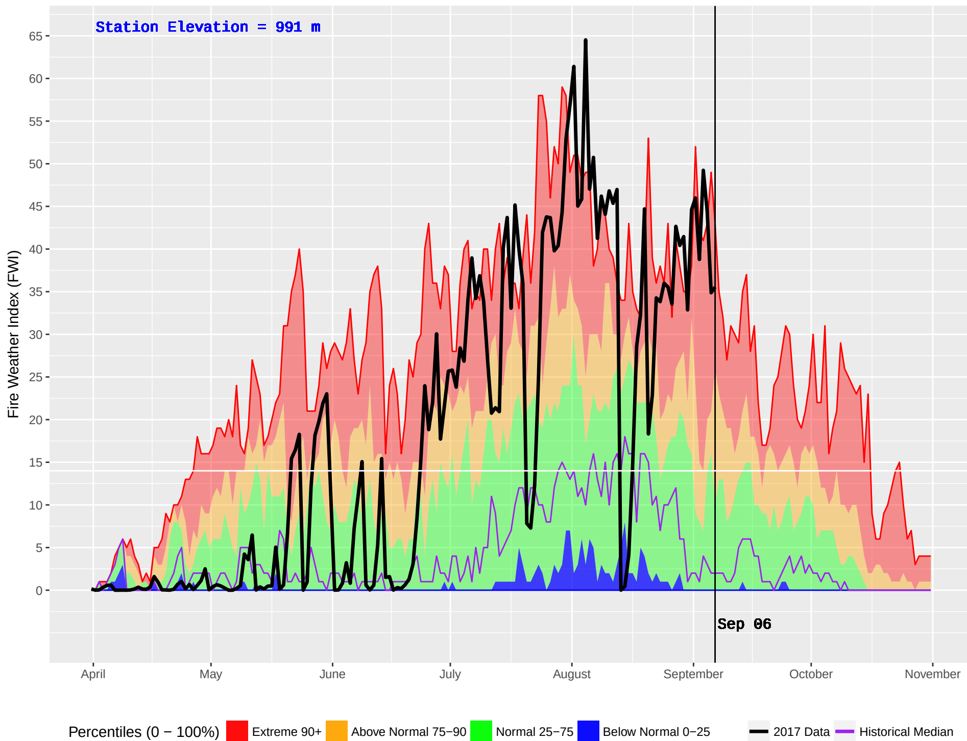
TROUT LAKE (387) : Historical (1987–2016) and Current (2017) Noon Fire Weather Index (FWI)
