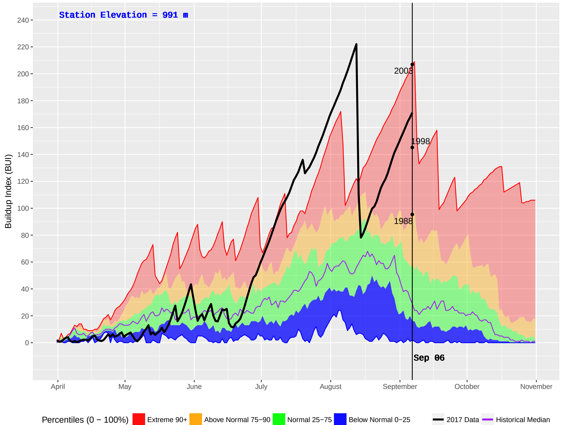
TROUT LAKE (387) : Historical (1987–2016) and Current (2017) Noon Buildup Index (BUI)
