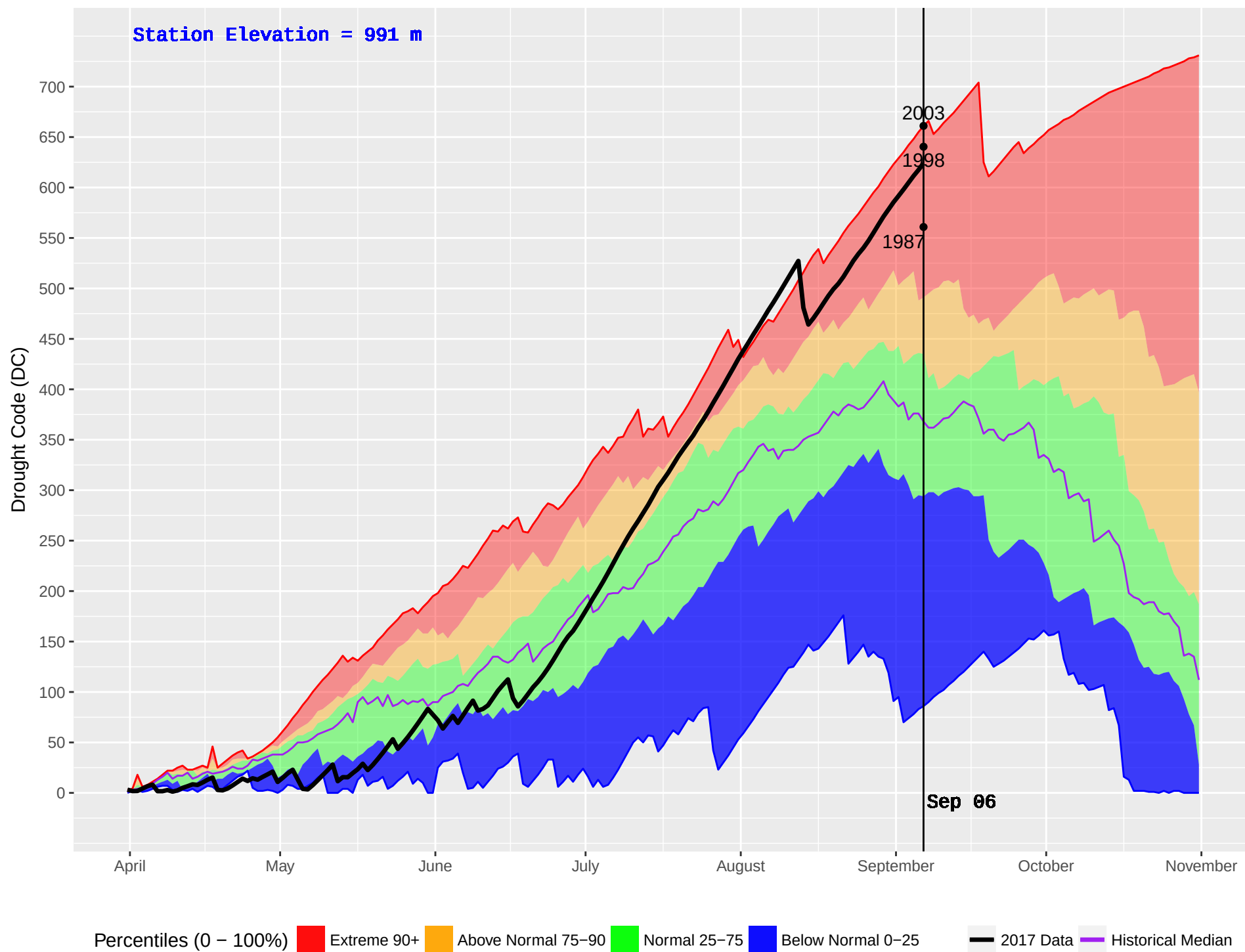
TROUT LAKE (387) : Historical (1987–2016) and Current (2017) Noon Drought Code (DC)
