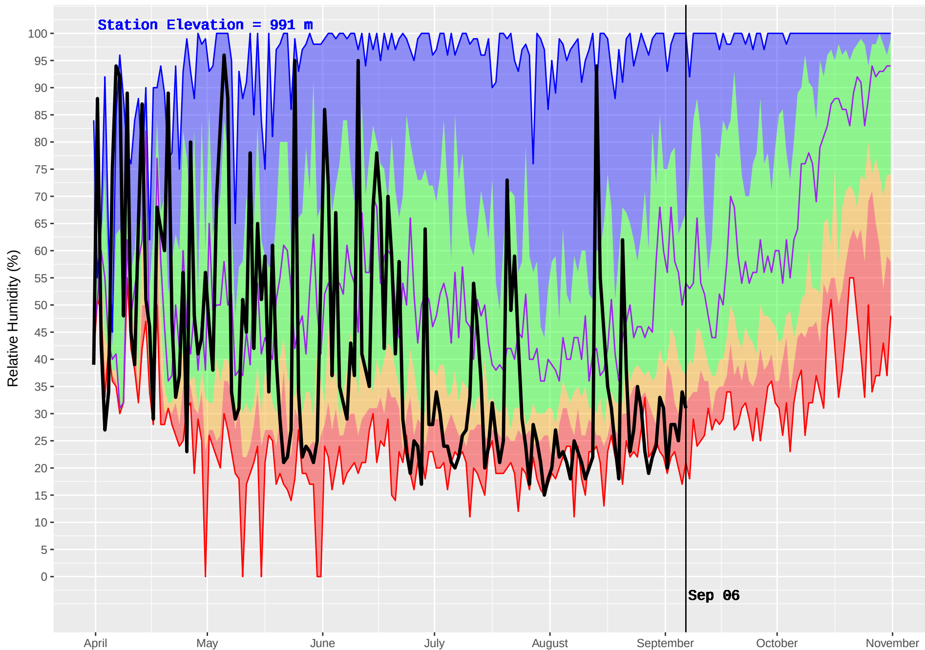
TROUT LAKE (387) : Historical (1987–2016) and Current (2017) Noon Relative Humidity
