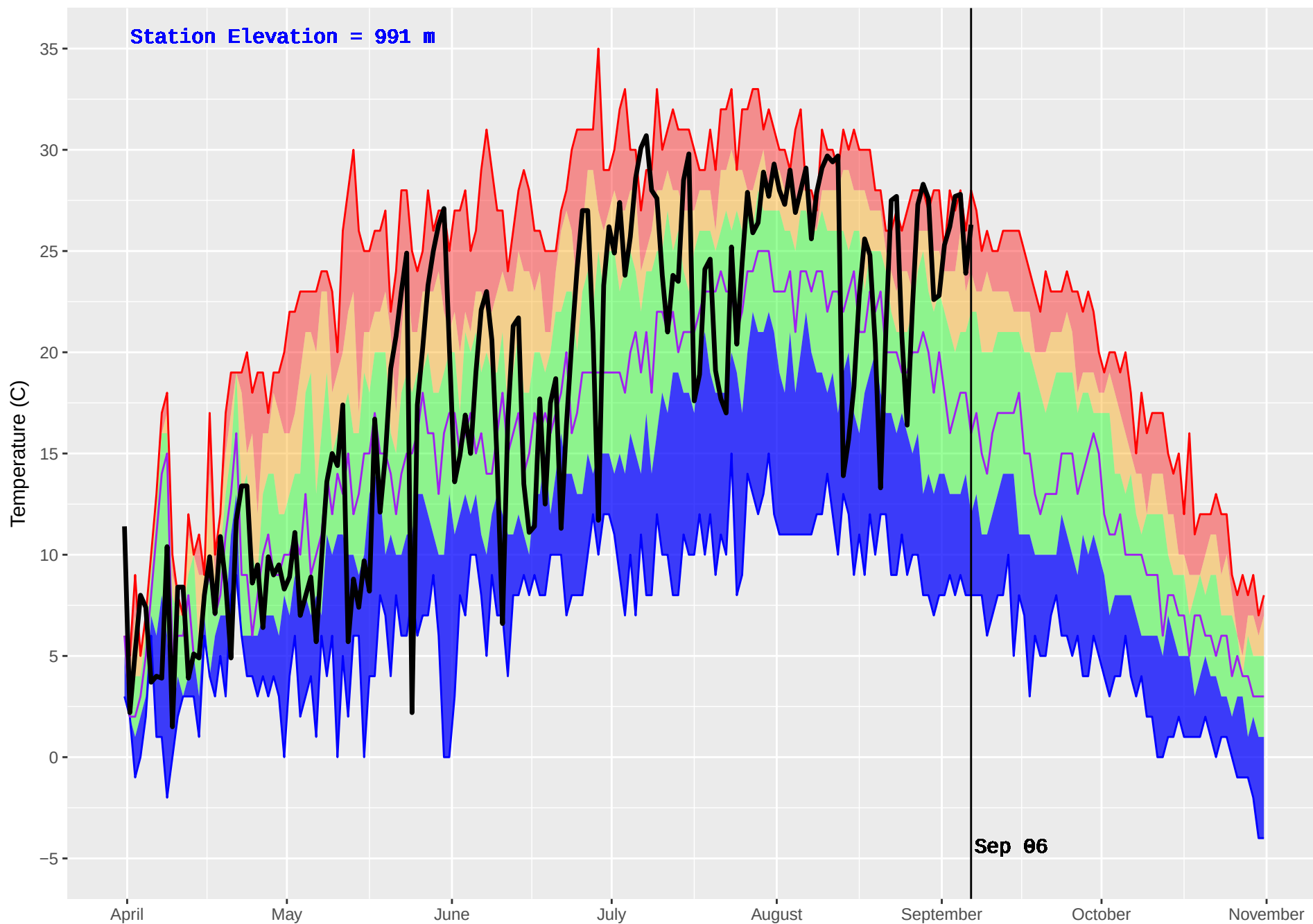
TROUT LAKE (387) : Historical (1987–2016) and Current (2017) Noon Temperature
